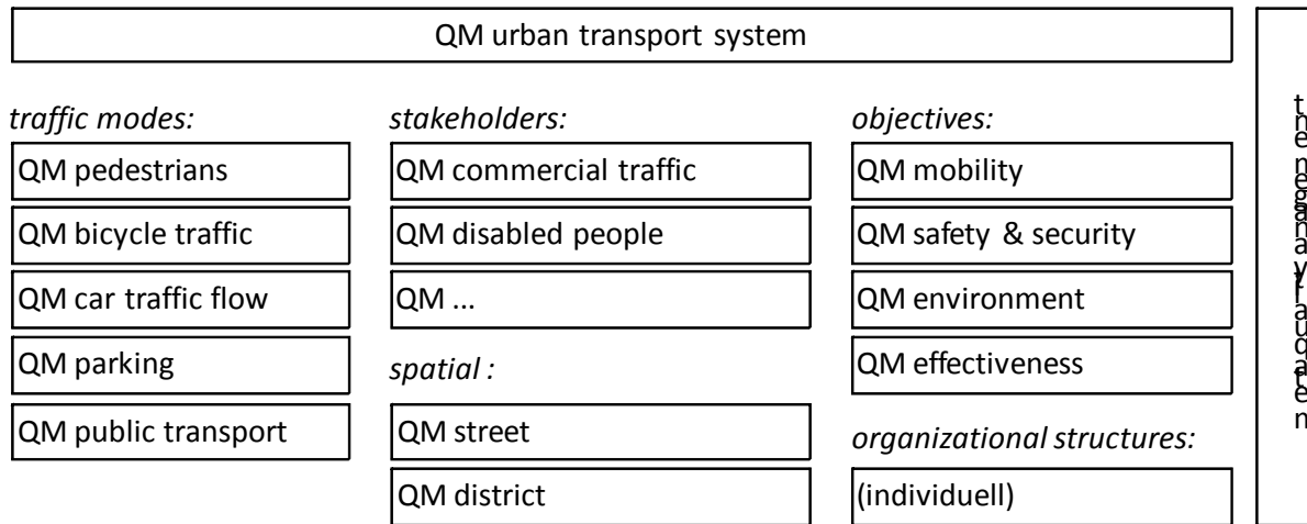
Figure 4 – Superordinate modules
