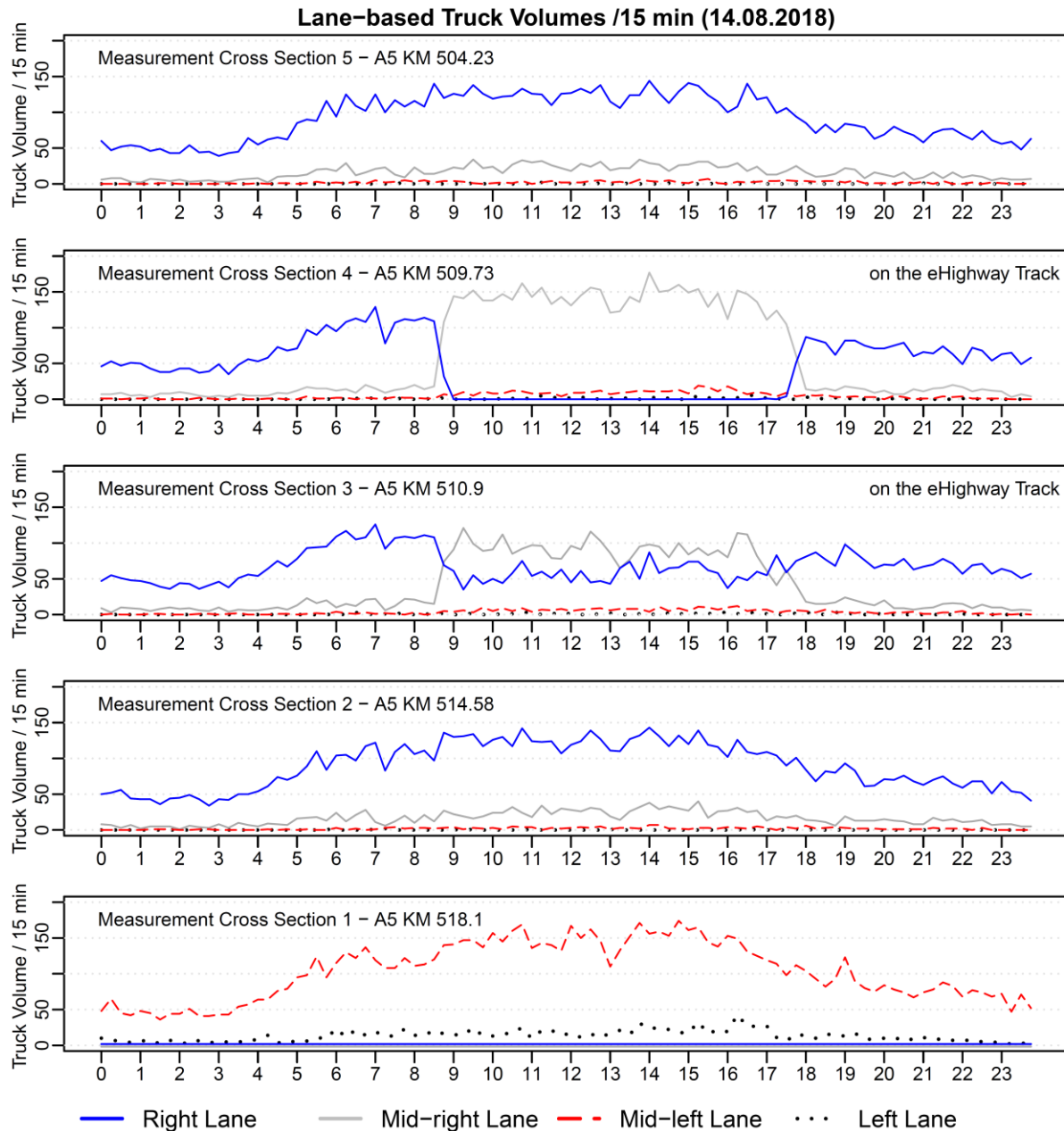
Figure 4: Lane-based Truck Volumes at Measurement Cross Sections on A5 North (14.08.2018)
